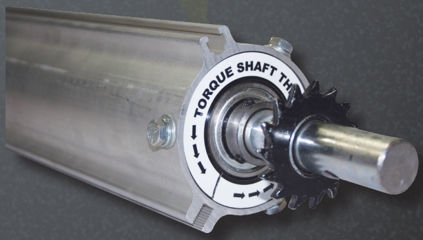
ROLLER BAR • P/N 1803805 Replaces Competitor P/N HR47002C
